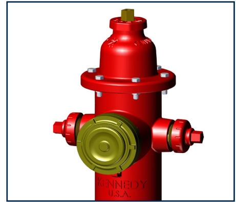
Storz Nozzle 5-1/4" Pumper Outlet Quick, universal 1/4 turn hose to hydrant connection for ease of operation.
