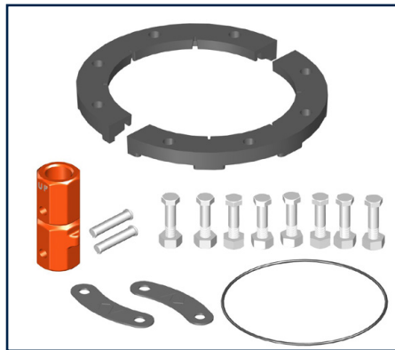
K8149 Collision Repair Kit Components to restore hydrant to service following a collision.
