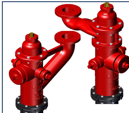
K81-DI 350 Monitor Hydrant & K81-AM Monitor Hydrant Provides the ability to mount a monitor nozzle in 3" or 4" flange pattern.
