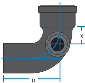
1/4 BEND w/ 2" HUB SIDE OPENING
