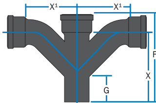
DOUBLE COMBINATION
