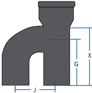
VENT BRANCH
