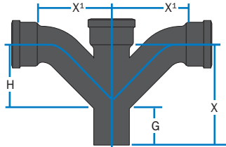
DOUBLE COMBINATION (SHORT TURN)
