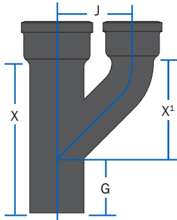
"H" BRANCH
