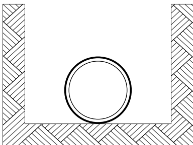
Type 1* Flat-bottom trench.† Loose backfill.
